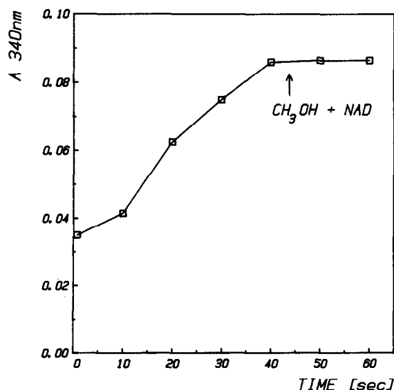
Fig.2. The rate of absorbance increase at 340 nm in methanol dehydrogenase after adding methanol (2 mM) and NAD + (2.5 mM) to the enzyme in 0.1 M tetrasodium pyrophosphate (pH 9.0), containing 0.12 M NH 4 Cl. The enzyme preparation used was the fraction eluted from DEAE-Sephacel, after removal of NADH dehydrogenase.
