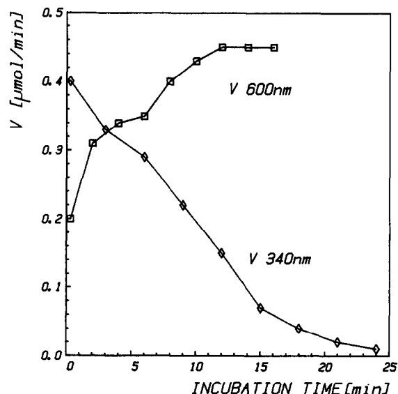
Fig.3. Methanol dehydrogenase activities during the incubation of the methanol dehydrogenase-containing fraction with the NADH dehydrogenase-containing fraction. NAD-dependent DCIP reduction ( v_{600nm} ) and the rate of absorbance increase at 340 nm ( v_{340nm} ) were measured as described in section 2. The fractions used were obtained from the DEAE-Sephacel column.
